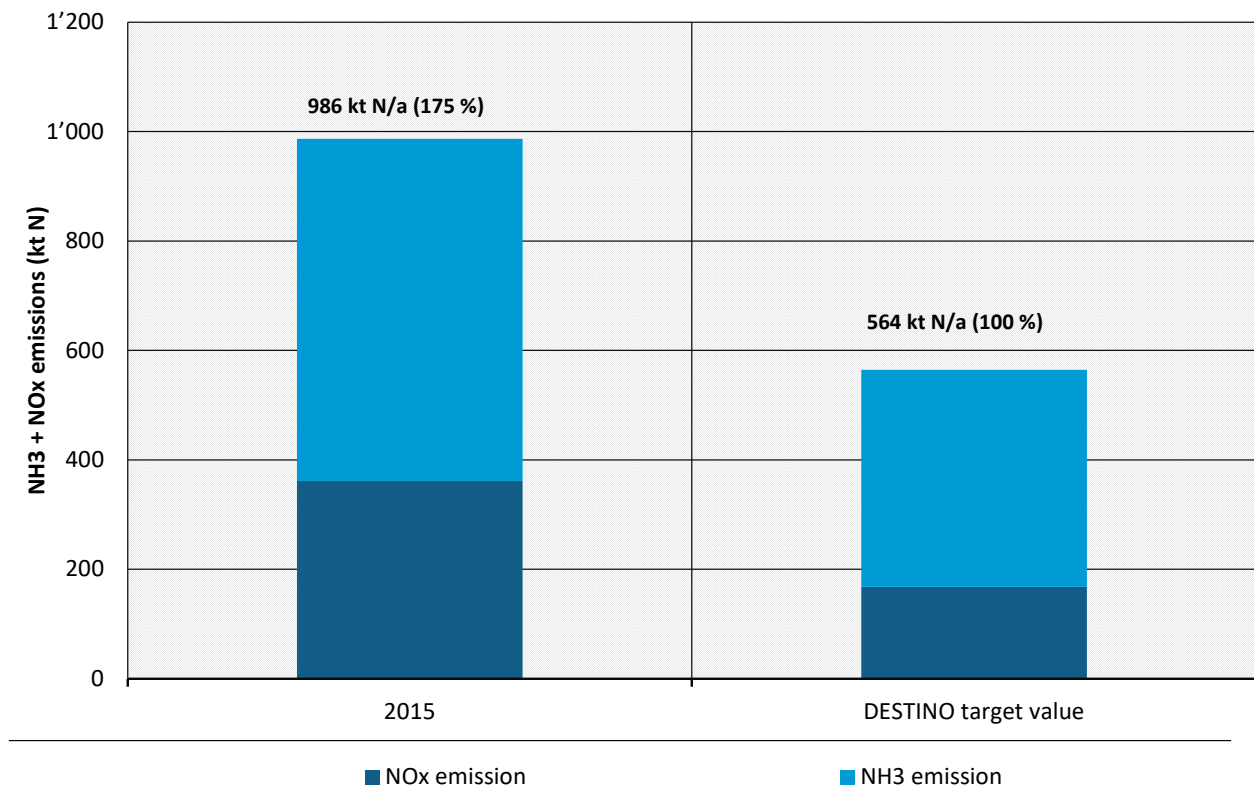
Figure 10: DESTINO-indicator terrestrial ecosystems / critical load, sum of NH 3 and NO x emissions. Current status (2015) and DESTINO target value.
