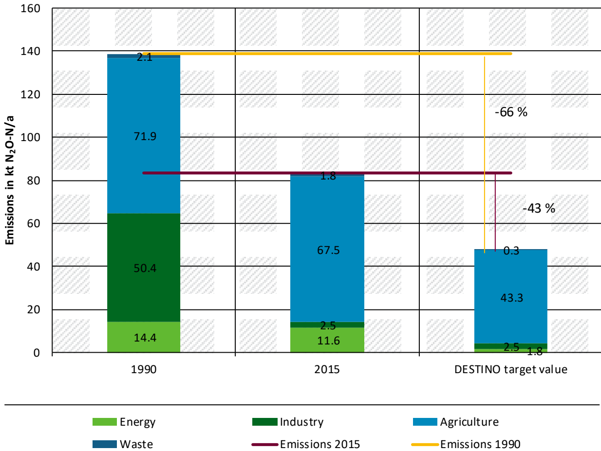
Figure 15: Nitrous oxide emissions according to sectors and DESTINO target value for the Climate sector.
