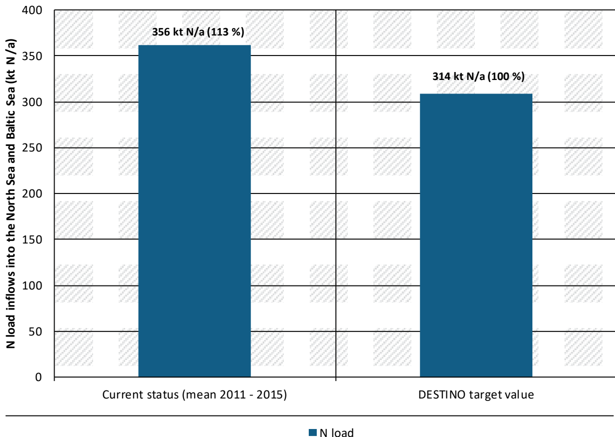
Figure 11: DESTINO-indicator Surface waters, N-load in inflows into the North Sea and Baltic Sea. Current status (annual mean 2011 - 2015) and DESTINO target value.
