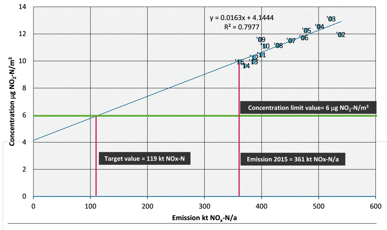
Figure 28: Regression of the 98 th percentile of the measured NO 2 ambient concentrations and the NO x emissions (national total) for the years 2002 to 2015
