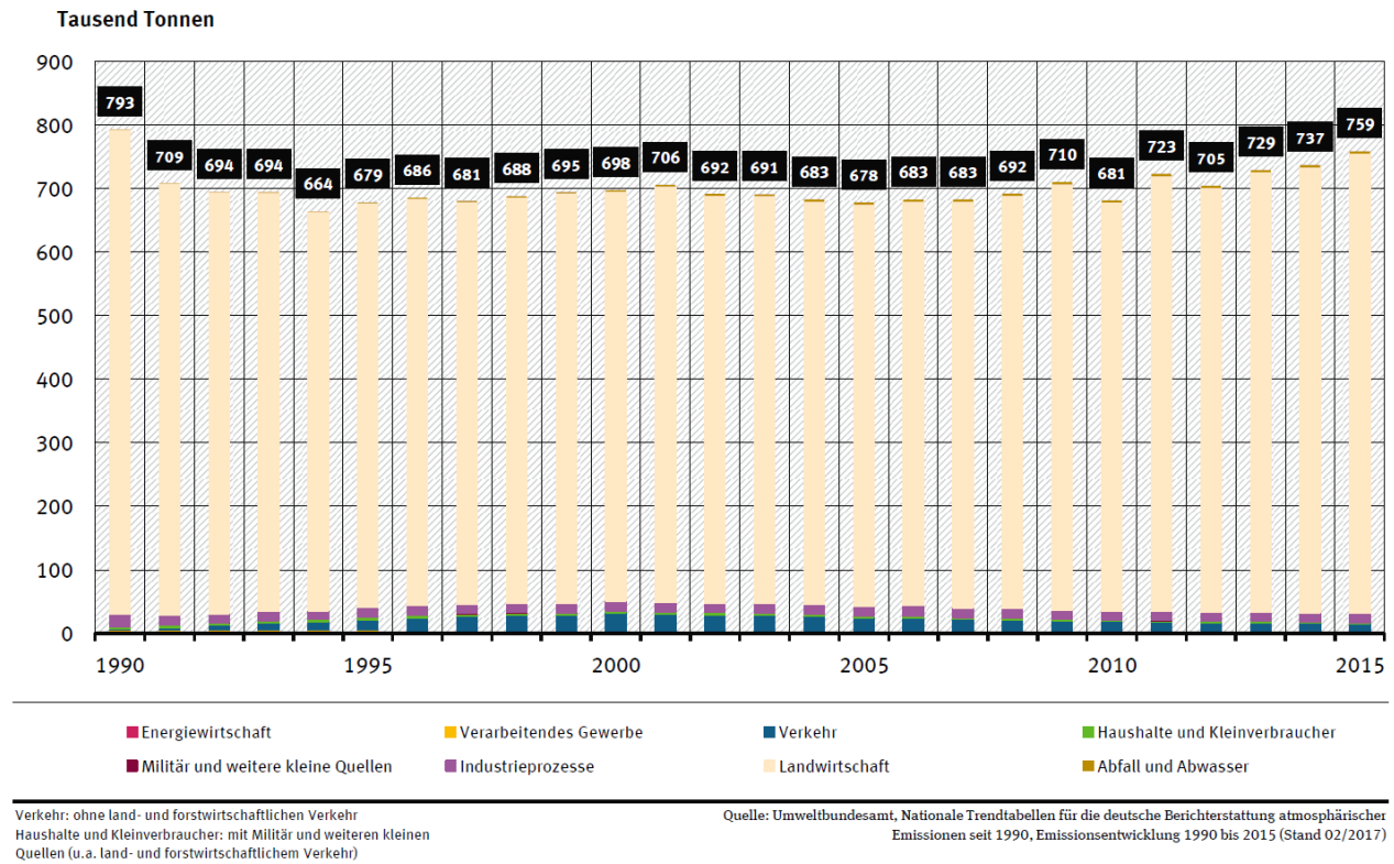
Figure 25: NH 3 emissions according to source (in 1000 t NH 3 ), as of 2017.
