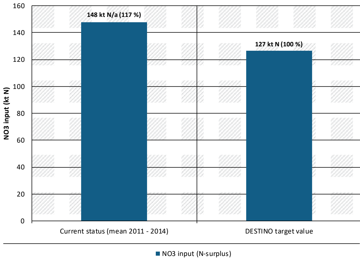
Figure 13: DESTINO-indicator Groundwater, N-surplus of the agricultural area in grid cells exceeding the threshold concentration. Current status (mean 2011 - 2014) and DESTINO-target value.
