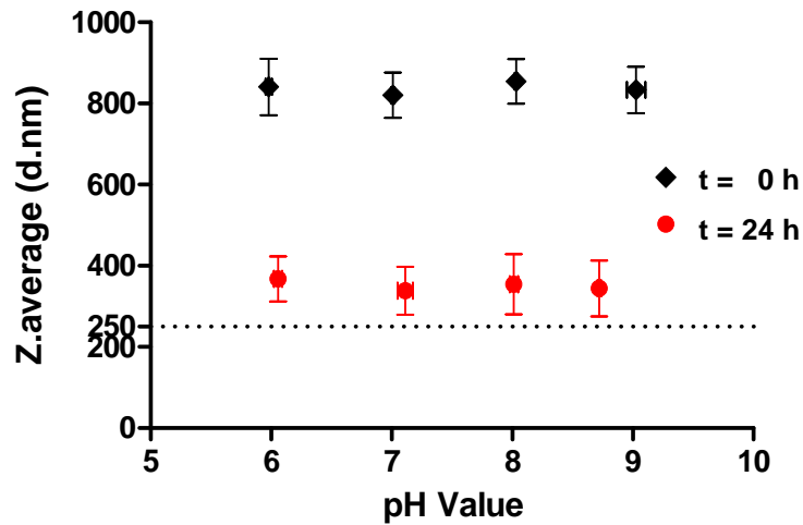
Figure 62: pH value dependent particle sizes of PC105 (100 mg/L) in 100 mL synthetic drinking water and 1 wt% SHP after sonication for 5 min. Error bars are SD. Measured at 0 h and 24 h; n = 3.
