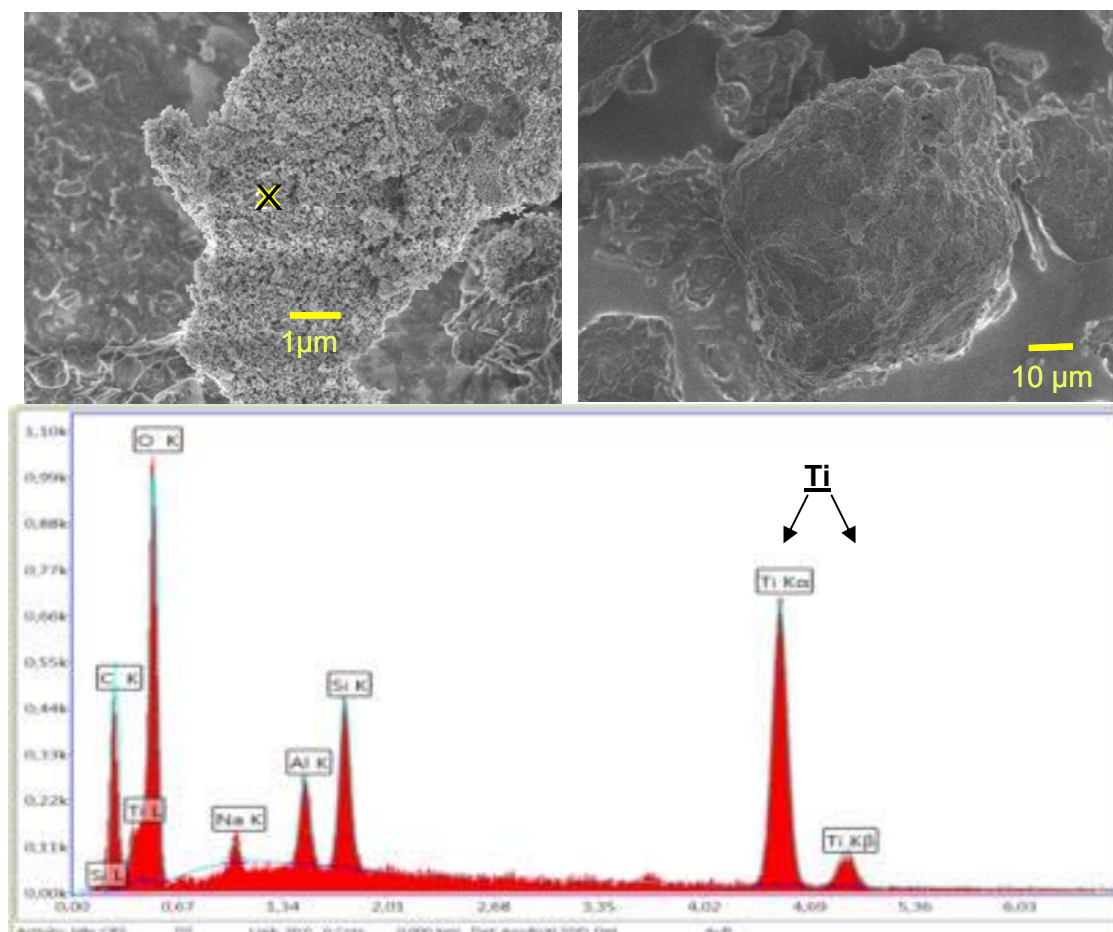
Figure 92: SEM / EDX scans of segment one of soil A06 treated with P25.
