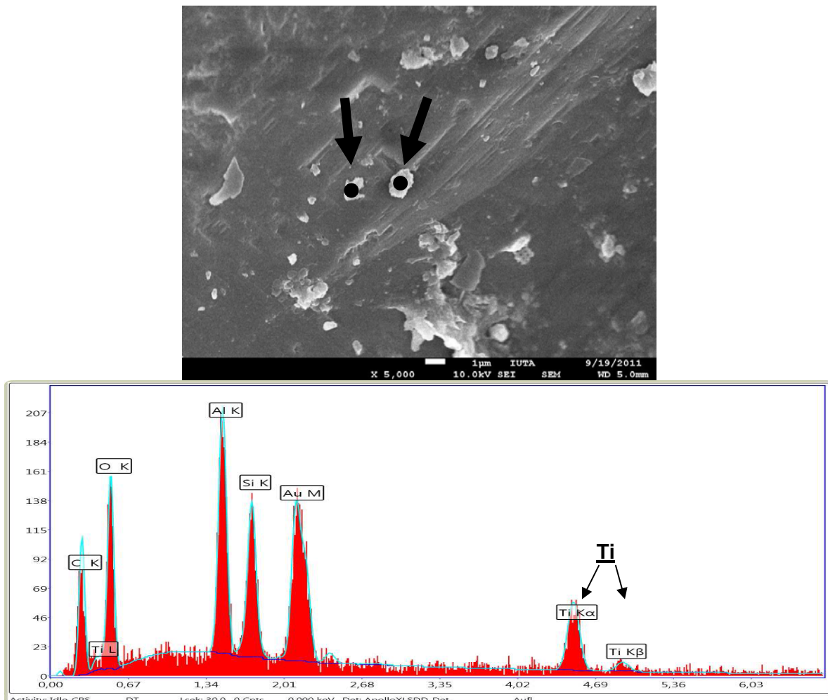
Figure 83: SEM / EDX scans of segment two of soil A04 treated with PC105.
