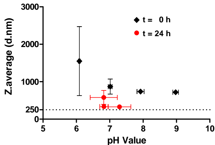
Figure 61: pH value dependent particle sizes of 100 mg/L PC105 in 100 mL DI after sonication for for 5 min (200 W). Error bars are SD. Measured 0 h and 24 h after sonication; n = 3.
