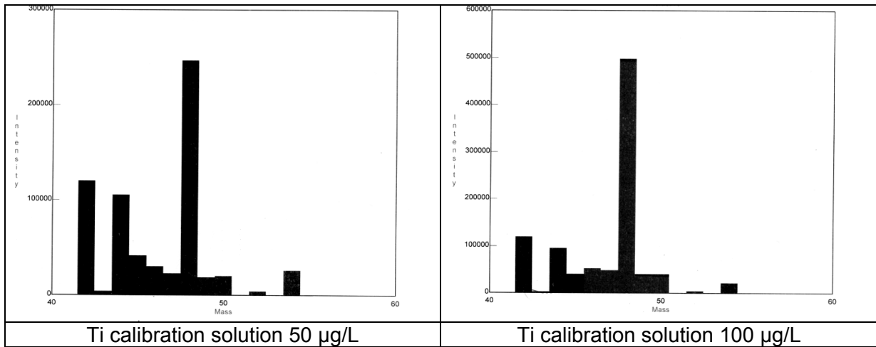
Figure 9: Counts for the 40 to 60 amu (atomic mass unit) analysing Titanium calibration solutions. A mass from 46 - 50 relate to Titanium.
