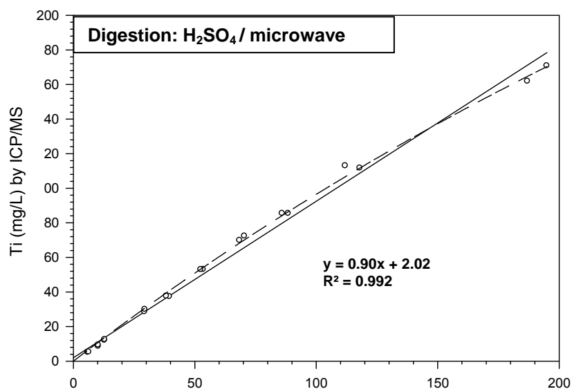
Figure 12: Comparison of Ti analysis by ICP/OES and ICP/MS. All samples were digested using the H 2 SO 4 /microwave method.
