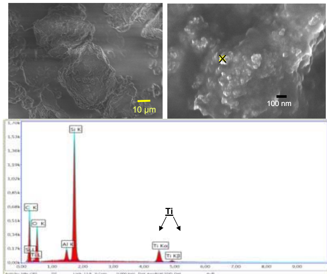
Figure 91: SEM / EDX scans of segment one of soil A06 treated with UV Titan M262.
